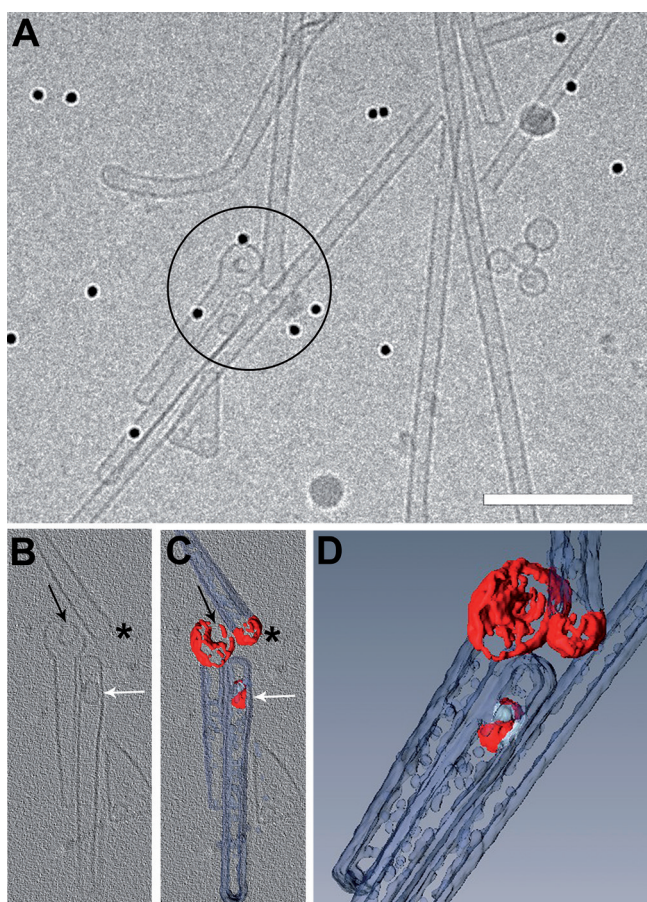
Figure 3. A) CryoTEM of a sample DOPC:1 (1:1; 1 \text{ mg mL}^{-1} each) in 10 \text{ mM aq. NaCl} after addition of 200 \text{ mM aq. NaCl} solution where the region of interest is highlighted with a circle (scale bar = 200 \text{ nm} ). The small black spherical objects are fiducial gold markers. B) Tomographic slice of reconstructed 3D area obtained by electron cryotomography. C) The same region of the reconstructed area (tomographic slice visible in the background) with the surface of the enclosed vesicles colored red and the surface of the nanotubes colored transparent blue. In both (B) and (C), the progress of inclusion of vesicles into nanotubes from the initially end-capped tube (*), through distorted vesicles attached to the end of a nanotubes (black arrow), to an included vesicle present inside a nanotube (white arrow), is shown. D) The same region as in (B) and (C) shown in a 3D reconstruction at a different viewing angle using the color scheme of (C), showing the dented geometry of the vesicle capping the end of the nanotube.
