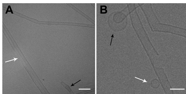
Figure 4. CryoTEM images of DOPC:1 (1:1 w/w, 1 \text{ mg mL}^{-1} each; in 10 \text{ mM aq. NaCl} ) to which a 200 \text{ mM aq. NaCl} solution is added to induce the formation of vesicles inside the nanotubes. The sample was then irradiated at \lambda = 365 \text{ nm} for A) 3 min and B) 6 min. In (A) the white arrow indicates a gap formed during irradiation and the black arrow indicates a vesicles still remaining inside the nanotube. In (B) the white arrow indicates a small vesicle released through a gap in the nanotube formed during the irradiation and the black arrow indicates a larger vesicle most probably present initially in the sample (see text for discussion). Scale bar in (A) = 100 \text{ nm} , in (B) = 50 \text{ nm} .
